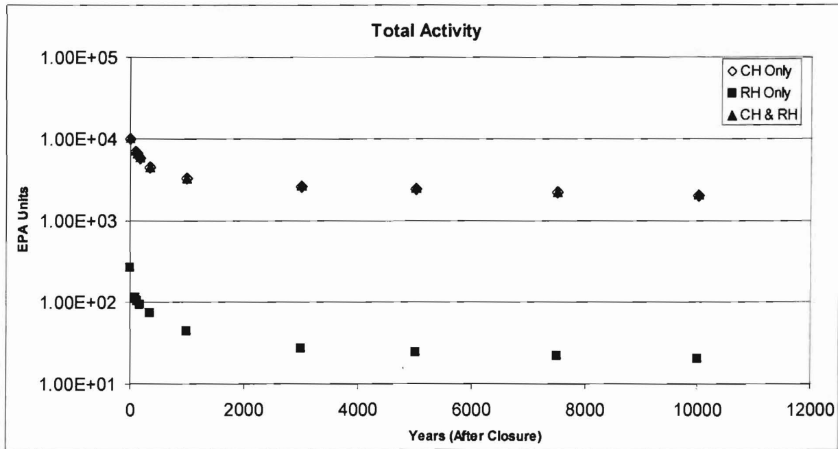
Figure 4. Total Activity vs. Time for RH and CH Waste.
