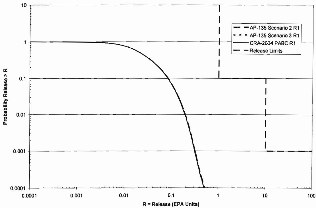
Figure 9. Mean Cuttings and Cavings Releases from SCPA Scenarios 2 and 3 and CRA-2004 PABC, Replicate 1.
