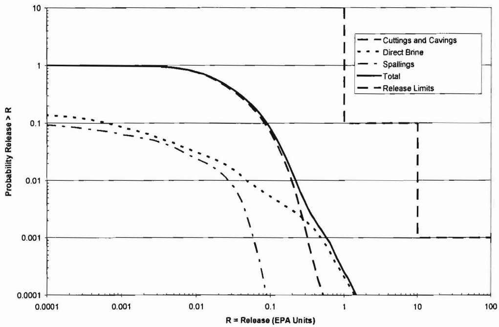
Figure A. 6. Mean Releases Mechanisms for SCPA Scenario 2, Replicate 1.
