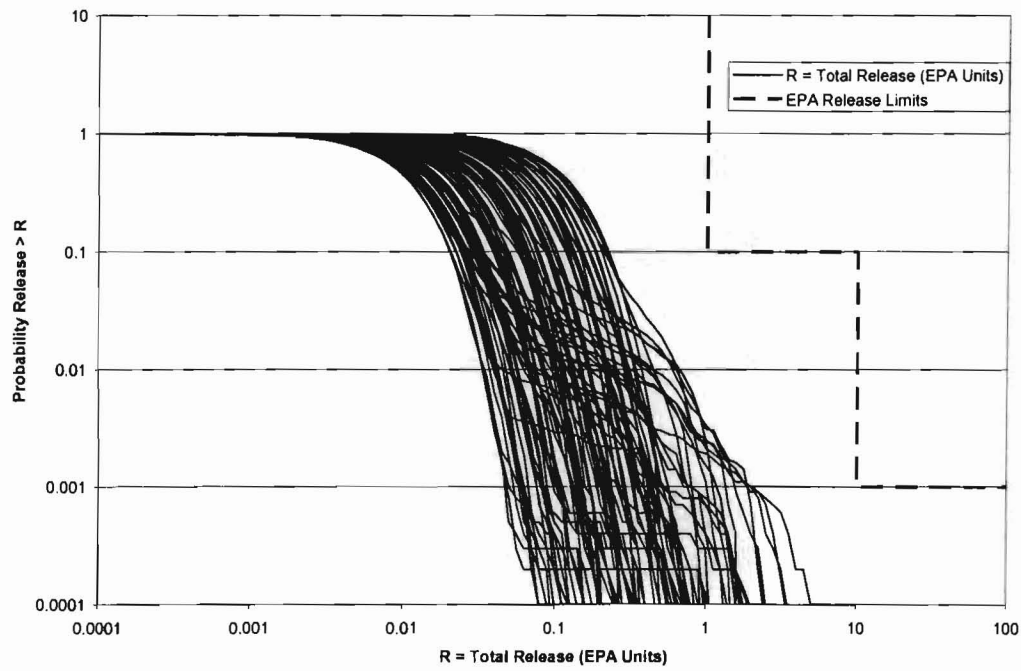
Figure A. 1. Total Releases for SCPA Scenario 2, Replicate 1.
