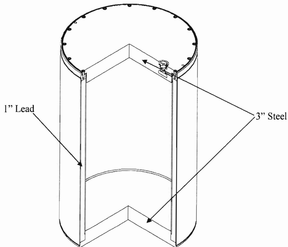
Figure 3. Isometric Exposed View of the Shielded Container.
