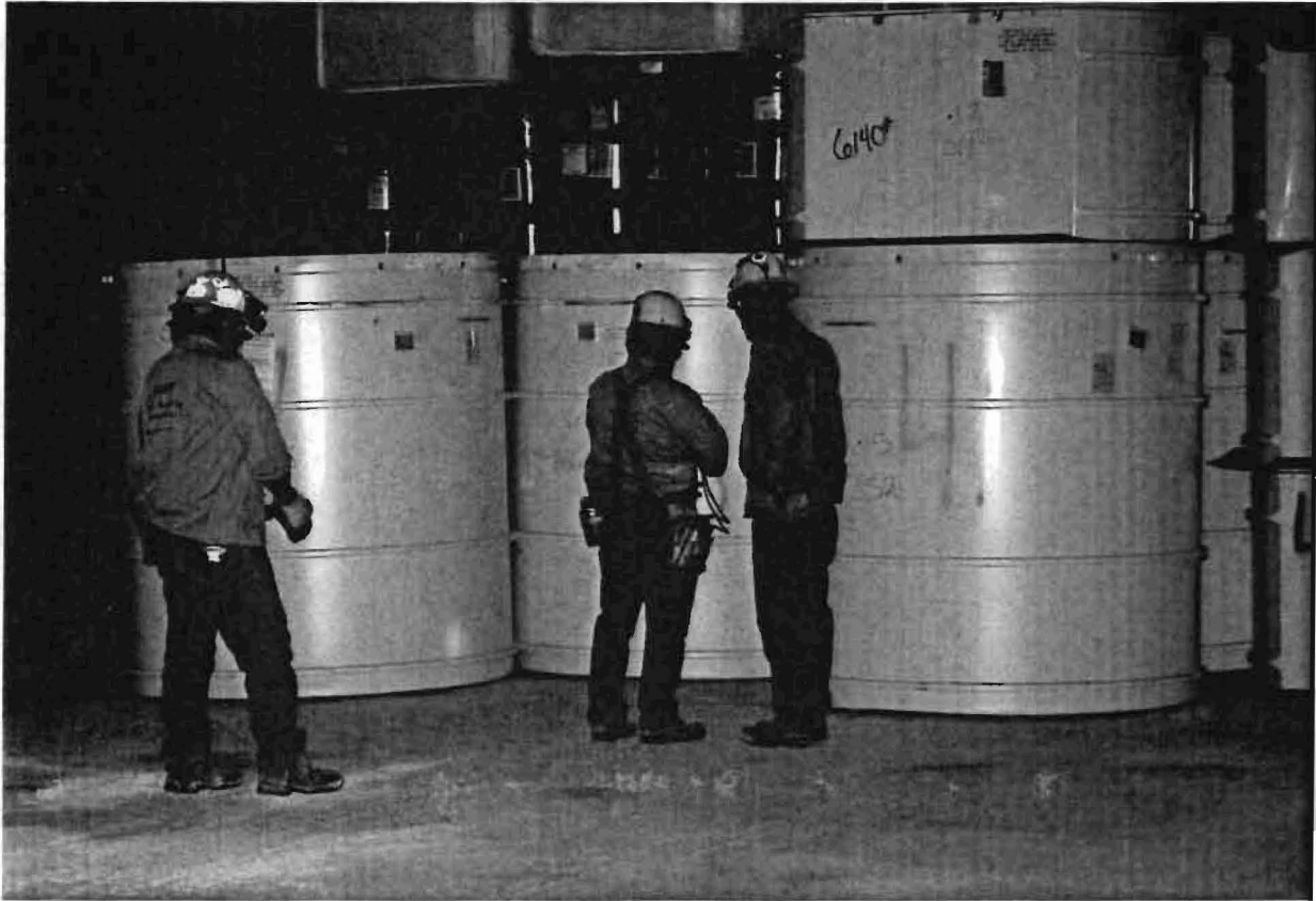
Figure 1. CH Waste Packaging Configurations in the WIPP. The black drums in the picture are 55-gallon drums shrink wrapped together into a 7-pack, and the containers on the floor are TDOPs. A SWB is placed on top of a TDOP on the right side of the picture. At the top of each stack is a supersack of MgO.
