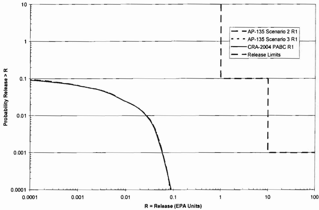
Figure 10. Mean Spallings Releases from SCPA Scenarios 2 and 3 and CRA-2004 PABC, Replicate 1.
