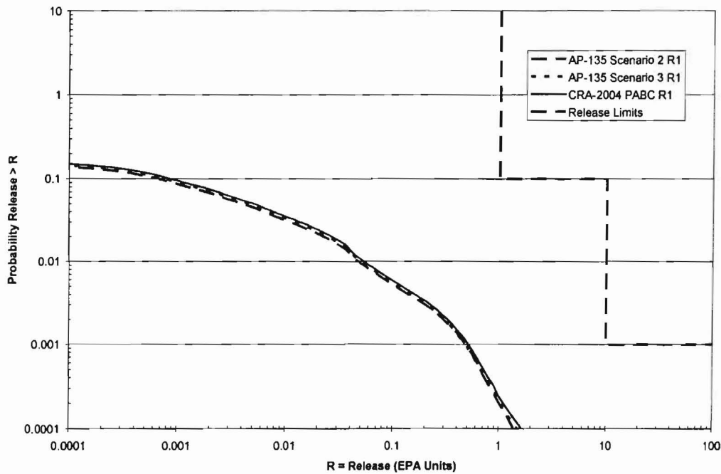
Figure 11. Mean DBRs from SCPA Scenarios 2 and 3 and CRA-2004 PABC, Replicate 1.
