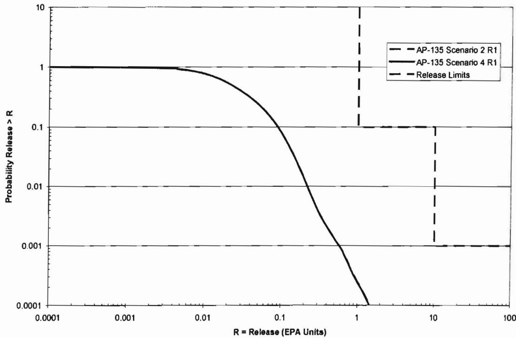
Figure 12. Mean Total Releases from SCPA Scenario 2 and Scenario 4, Replicate 1.
