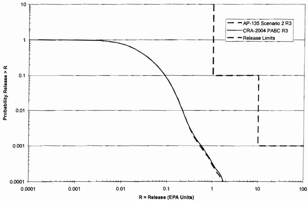
Figure A. 5. Mean Total Releases from SCPA Scenario 2 and CRA-2004 PABC, Replicate 3.
