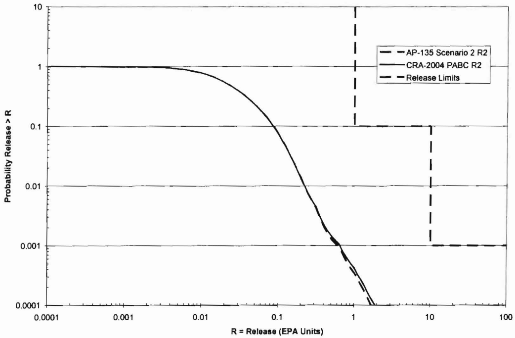
Figure A. 4. Mean Total Releases from SCPA Scenario 2 and CRA-2004 PABC, Replicate 2.
